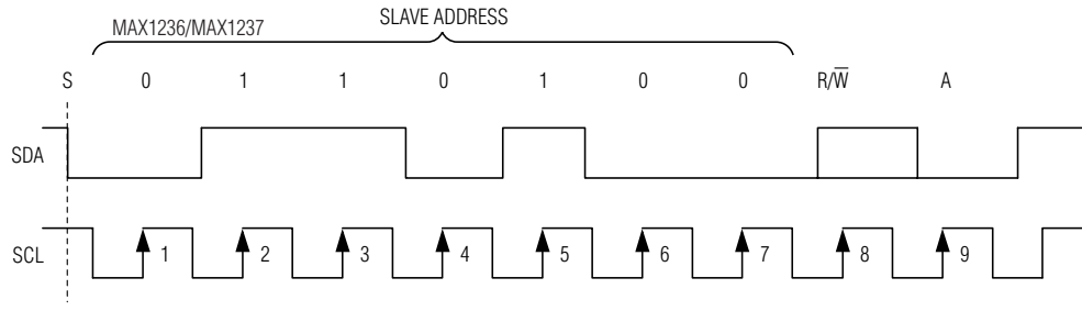
Figure 7. MAX1236/MAX1237 Slave Address Byte
